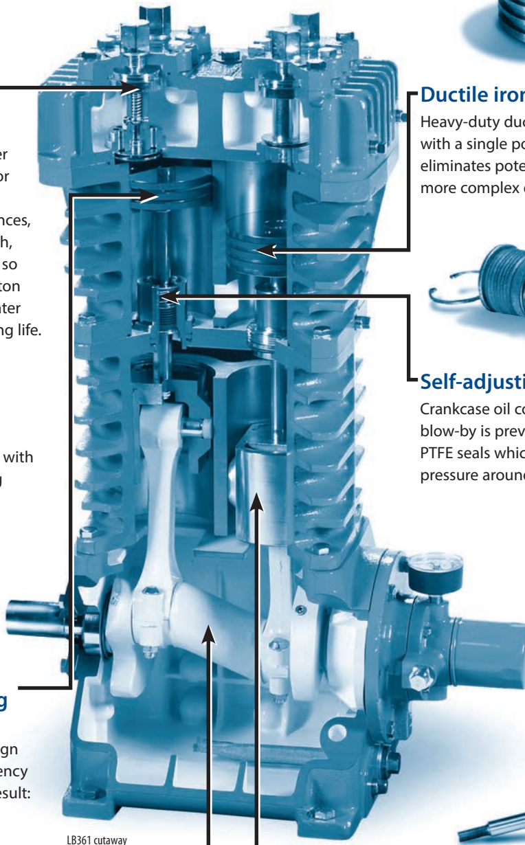
LB361 cutaway
