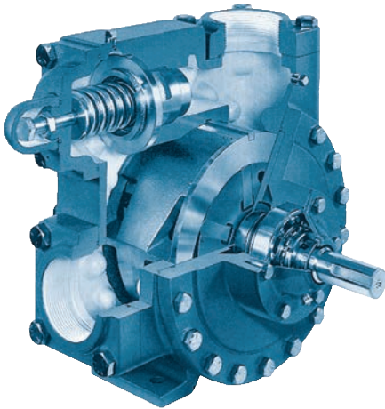
LGLD4 cutaway
